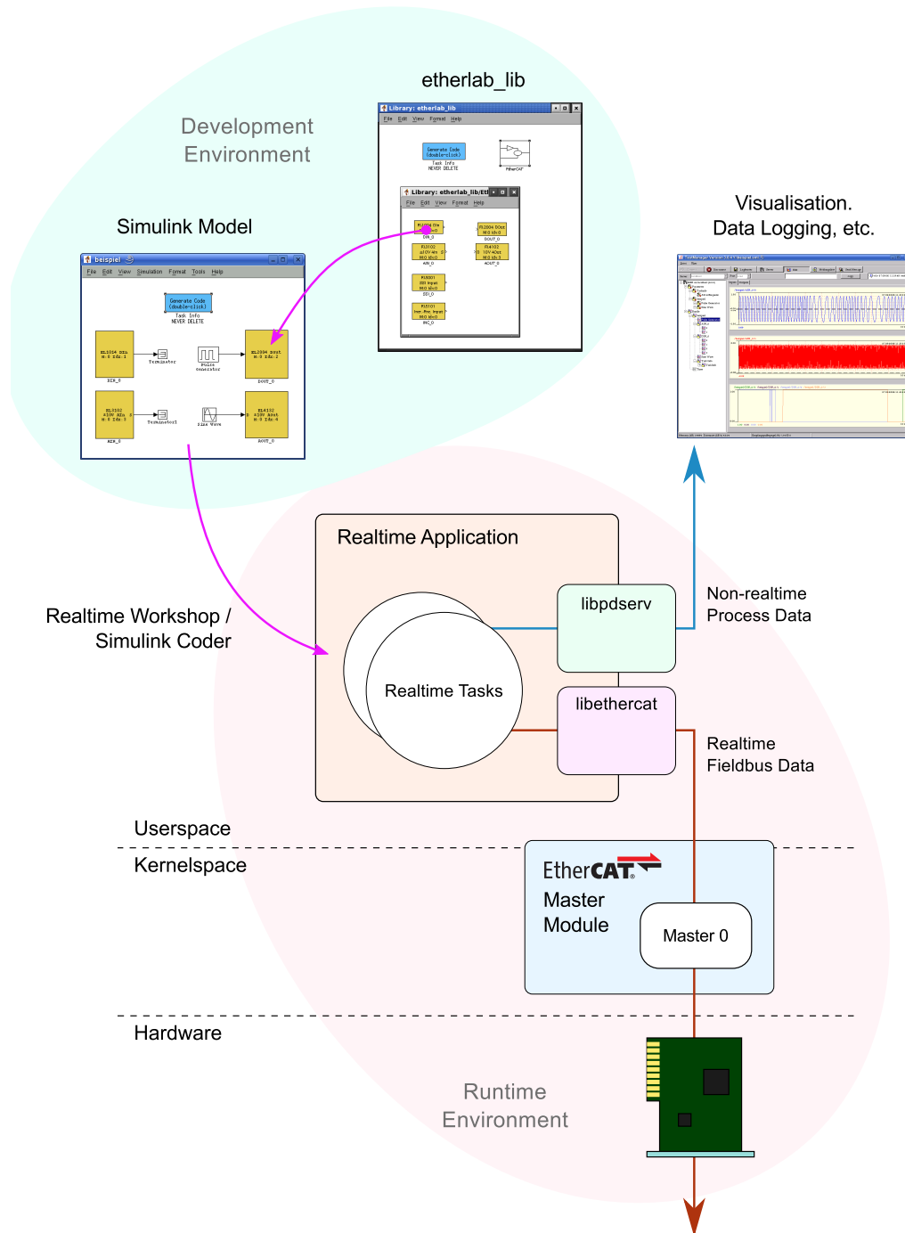
Figure 1: EtherLab Architecture
